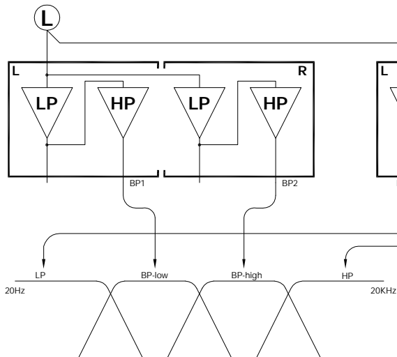
CROSSOVER #1 SPECIALLY MODIFIED 10B-LR, 10B-STD or 10B-SUB DUAL CHANNEL BAND PASS
