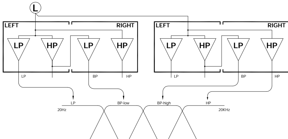
CROSSOVER #1 10B-LR, 10B-STD or 10B-SUB 3-Way Mono mode
