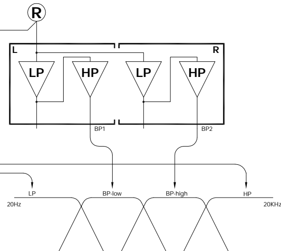
CROSSOVER #3 SPECIALLY MODIFIED 10B-LR, 10B-STD or 10B-SUB DUAL CHANNEL BAND PASS
