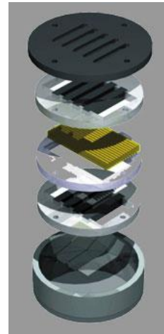
Tweeter A.D.A.M. Audio A.R.T. Compact Monitor
